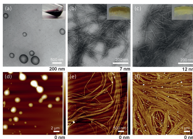
Figure 5. TEM images (a and b) and AFM height images (d and e) of NDI-Y acceptor and 1,5-DAN donor mixture (1:1) before (a and d) and after (b and e) exposure to thermolysin for 24 hours. The corresponding TEM (c) and AFM (f) images of the charge-transfer hydrogel of NDI-Y acceptor and 2,6-DAN donor mixture (1:1) after exposure to thermolysin for 24 hours. Insets in (a–c) show the digital photographs of the corresponding gel/sol samples.
